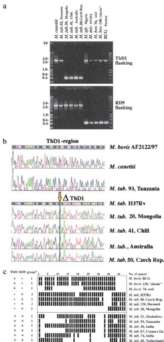
Fig. 1. (A) Amplicons obtained from strains that have the indicated genomic region present or deleted. Sizes of amplicons in each group are uniform. Numbers correspond to strain designation used in refs. 8 and 9. (B) Sequences in the Tbd1 region obtained from strains of various geographic regions. Numbers correspond to strain designation used in refs. 8 and 9. (C) Spoligotypes of selected M. tuberculosis and M. bovis strains. Numbers correspond to strain designation used in refs. 8 and 9. *, groups based on katG 463 / gyrA 95 sequence polymorphism defined by Sreevatsan et al. (2).
